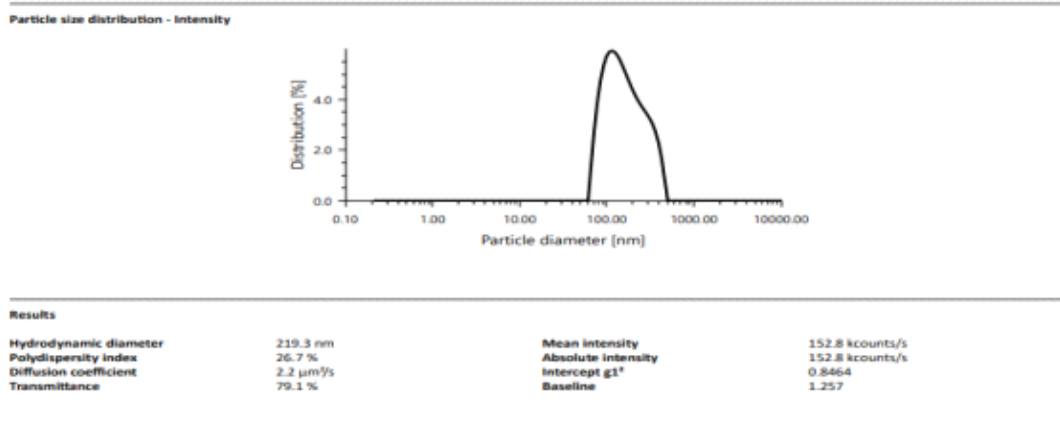
Fig. 1 : Dynamic light scattering (DLS) analysis of the phytosomal formulation showing a unimodal particle size distribution with an average hydrodynamic diameter of 219.3 nm and a polydispersity index (PDI) of 26.7
