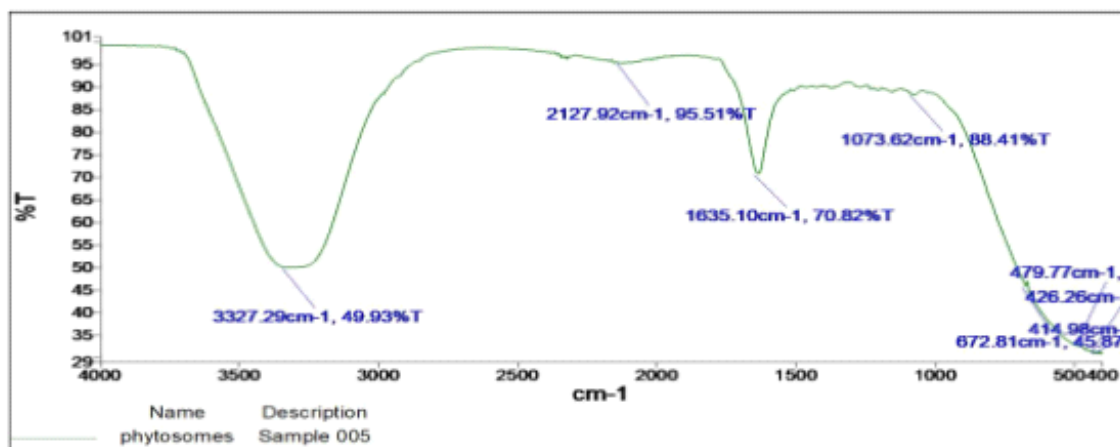
Fig. 4-FTIR spectrum of the phytosomal curcumin complex
